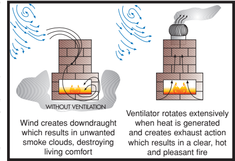
The positive extraction created by the Chimney Champ's rotating dome, ensures a smokeless and efficient fire.
